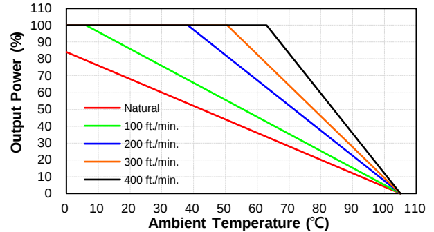
CQB100W14-72S15, 24, 28, 54 Derating Curve without Heatsink (Vin=72V)
