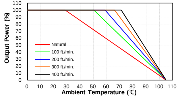
CQB100W14-72S05, 12 Derating Curve with Heatsink QBL127 (Vin=72V)
