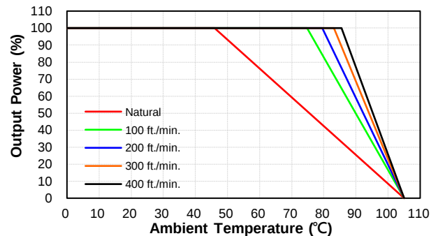
CQB100W14-72S15, 24, 28, 54 Derating Curve with Heatsink QBT210 (Vin=72V)
