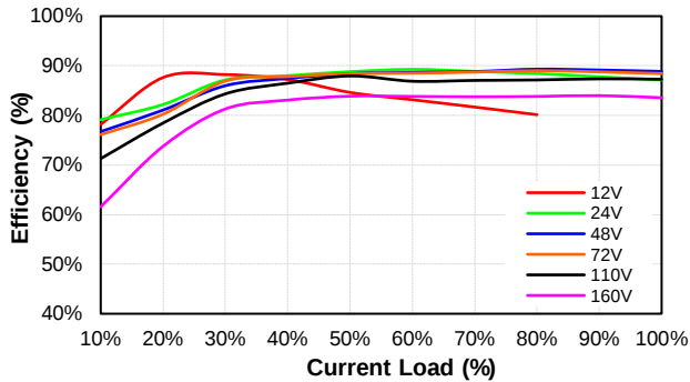
CQB100W14-72S05 Eff Vs Io @25 Deg. C
